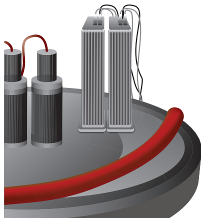
MXE pyrometers mounted side-by-side on tool
